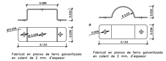
Brida per pal rectangular
