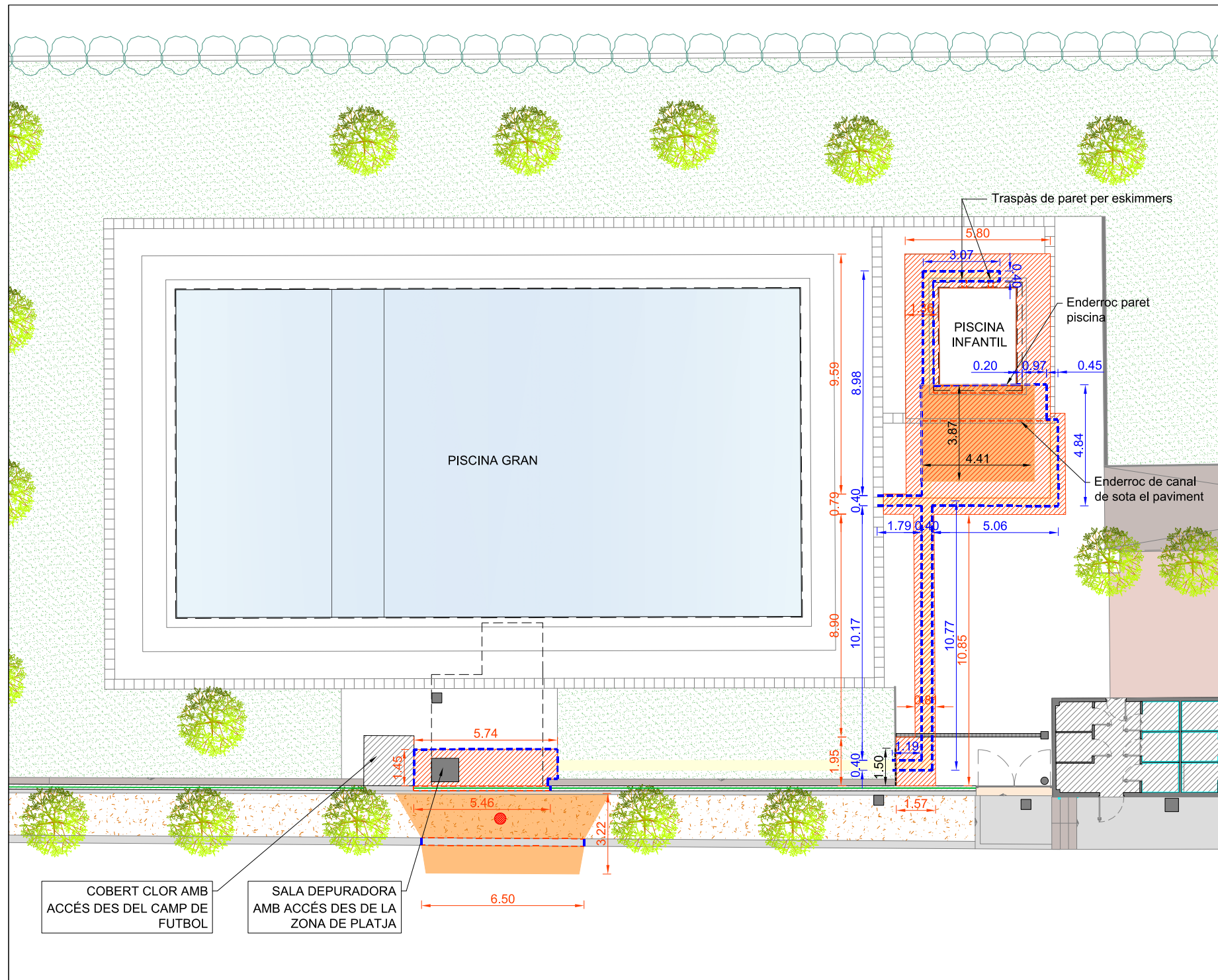
PLANTA GENERAL E/1:200
