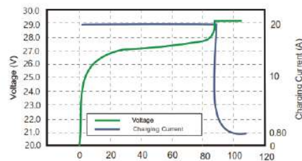
CHARGING CHARACTERISTICS @0.5C, 25°C
