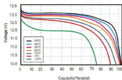
DISCHARGE CAPACITY at VARIOUS TEMPERATURES DISCHARGE @1C
