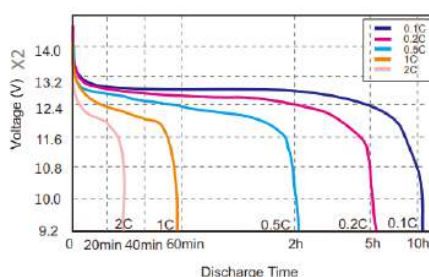
Different Rate Discharge Curve @25°C
