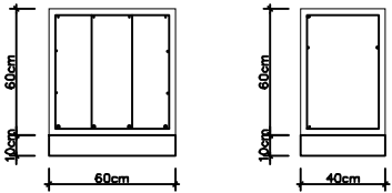
DETALLS SABATES CORREGUDES Escala 1/20
