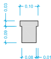
Montant pedra artificial
