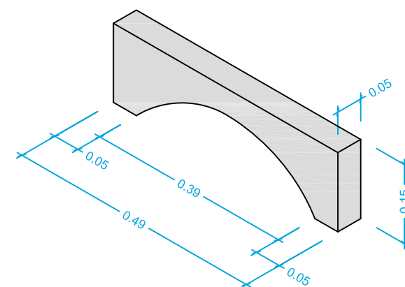
Cornisa central
