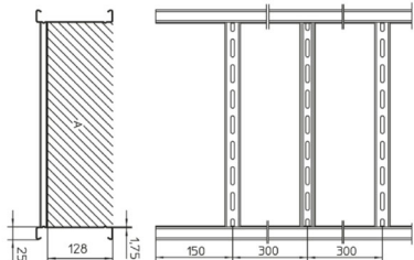
DETALL SAFATA MODEL PUK WPL150
