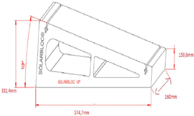
Dimensions SolarBloc
