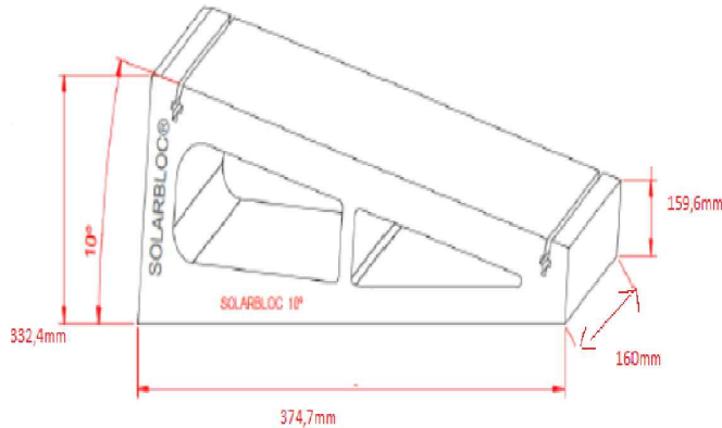
Dimensions SolarBloc
