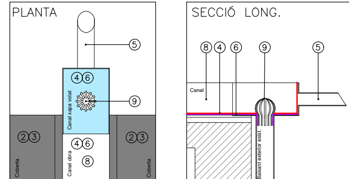
DETALL C –CANAL INT, BONERA, GARGOLA – E:1/20
