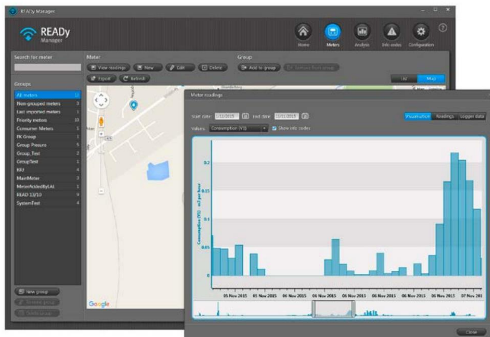
Figura 5. Ready Manager
