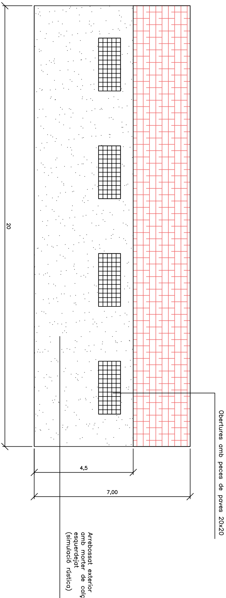
FAÇANA PRINCIPAL
