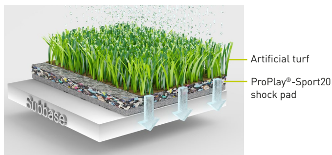
Artificial turf system with ProPlay®-Sport shock pad
