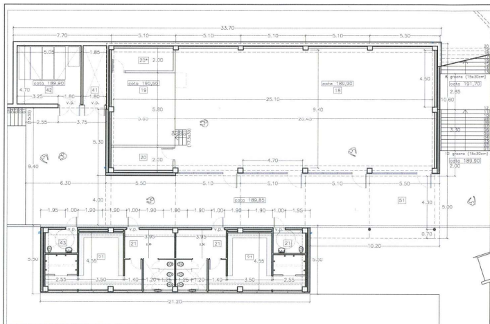
PLANTA BAIXA (tall cota 191.90)
