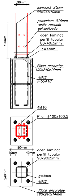
Arrencada pilar Tub 100x100.5
