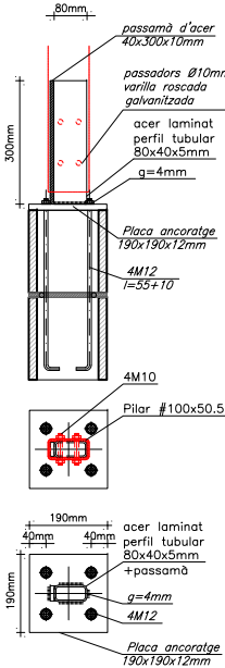
Arrencada pilar Tub 100x50.5
