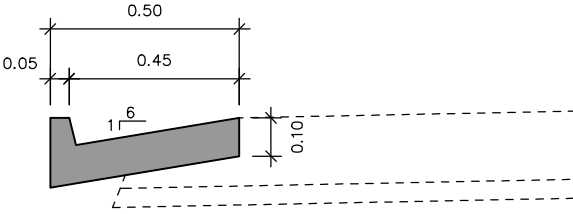
CUNETA TTR-50 E:1/20
