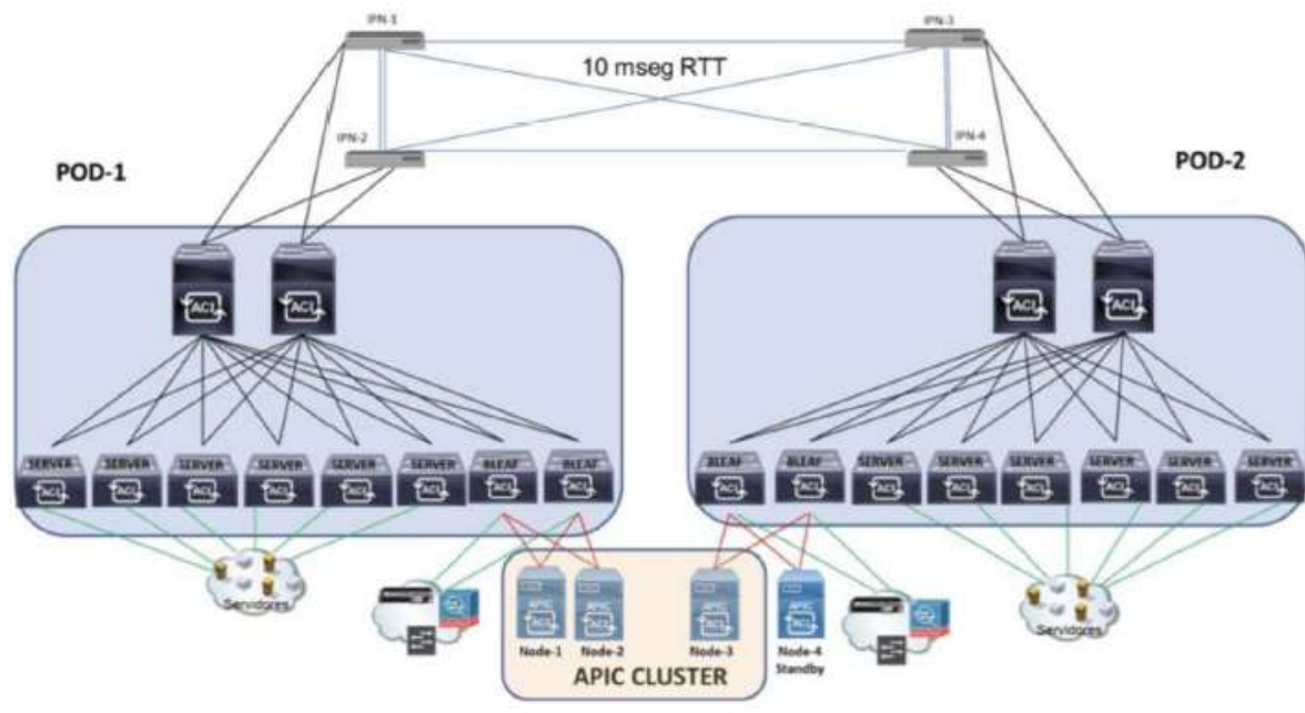
Figura 6: Arquitectura Multi-Pod
