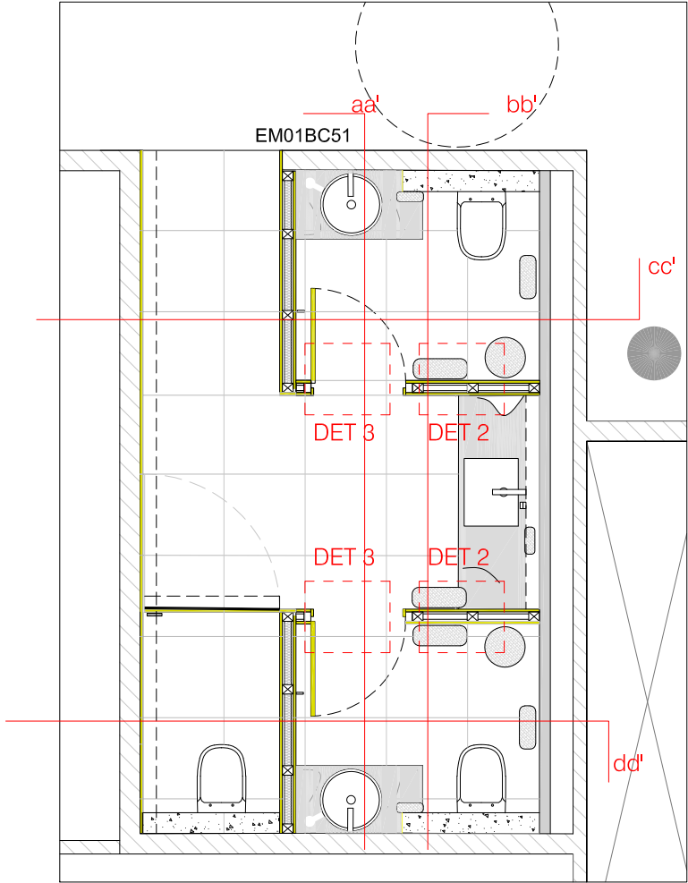
Planta Servei Higienic EM01BC51 e: 1/50 EM01BC31
