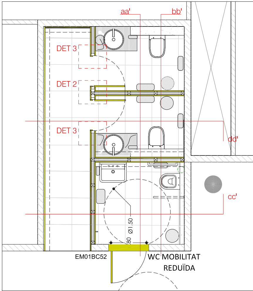
Planta Servei Higienic EM01BC52 e: 1/50 EM01BC32
