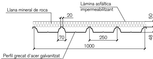
DETALL COBERTA DECK
