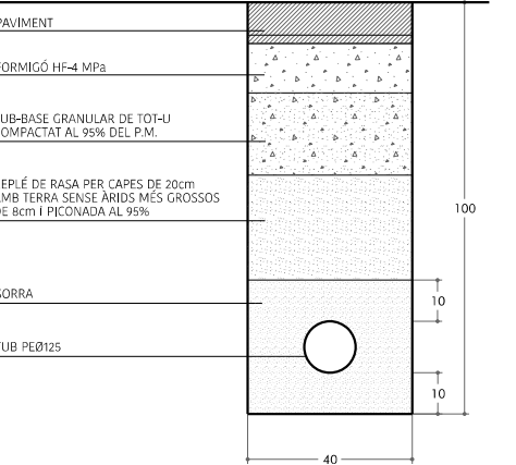
DETALL RASA - AIGUA POTABLE
