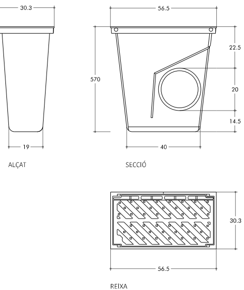
EMBORNAL - PLUJANES
