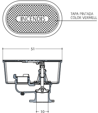
HIDRANT DN 100 - AIGUA POTABLE
