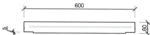
TAPA 500X600X60
