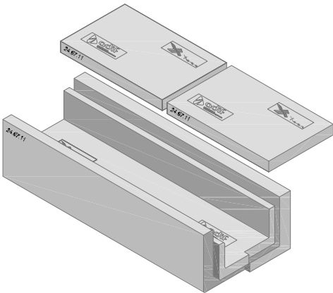
TAPA 500x287x60
