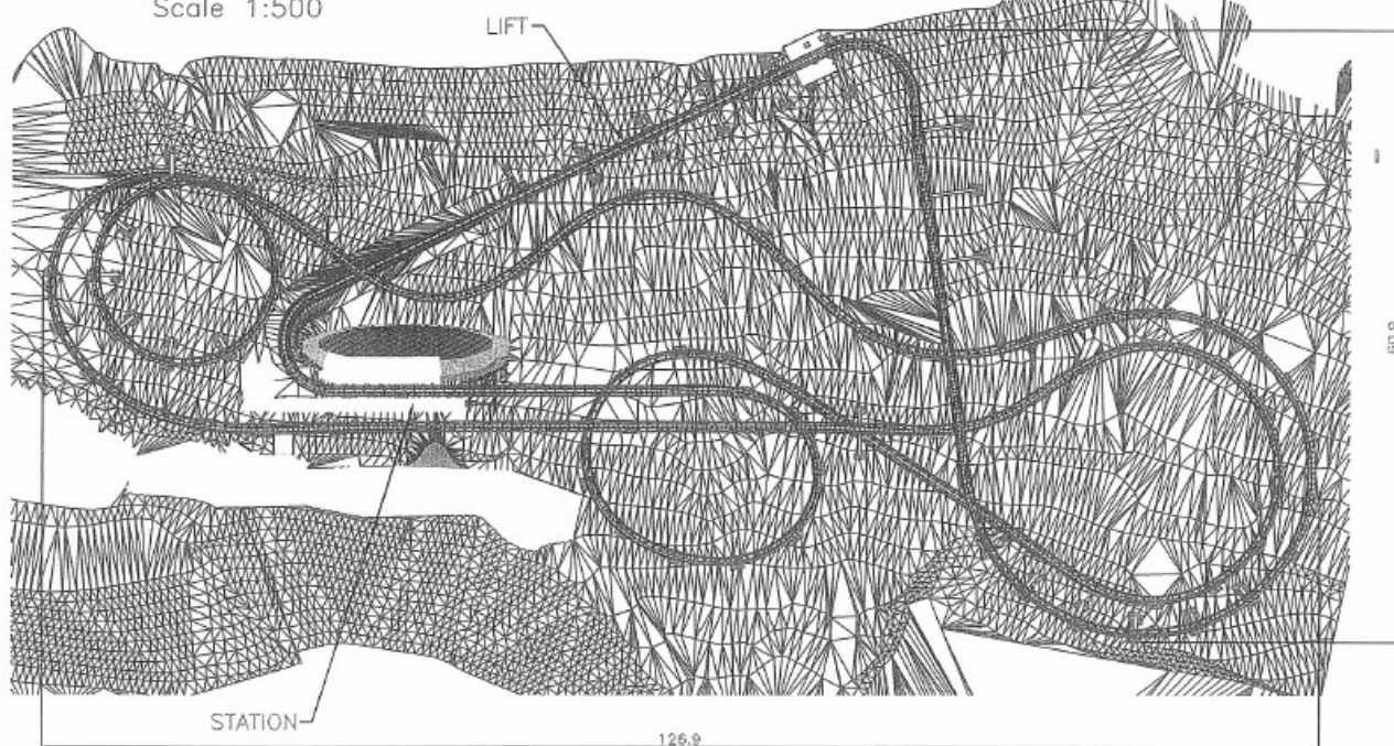
Topview Scale 1:500
