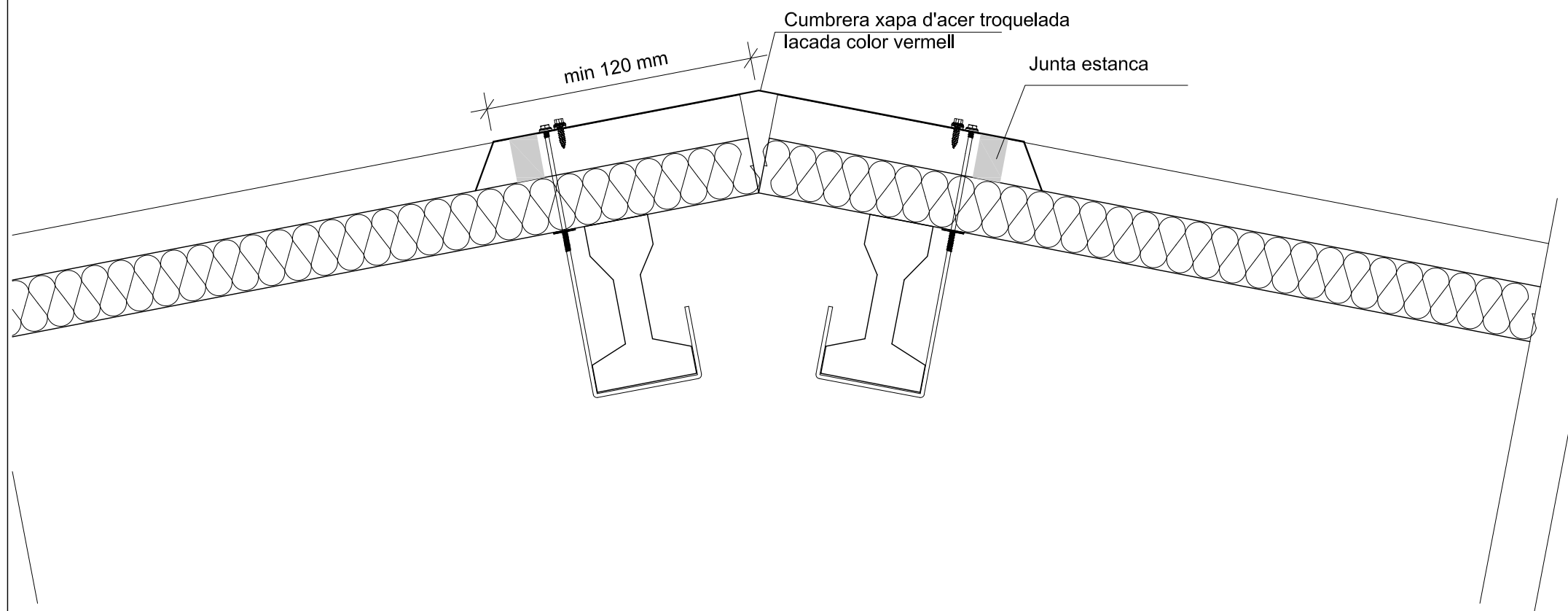
DETALL CARENER
