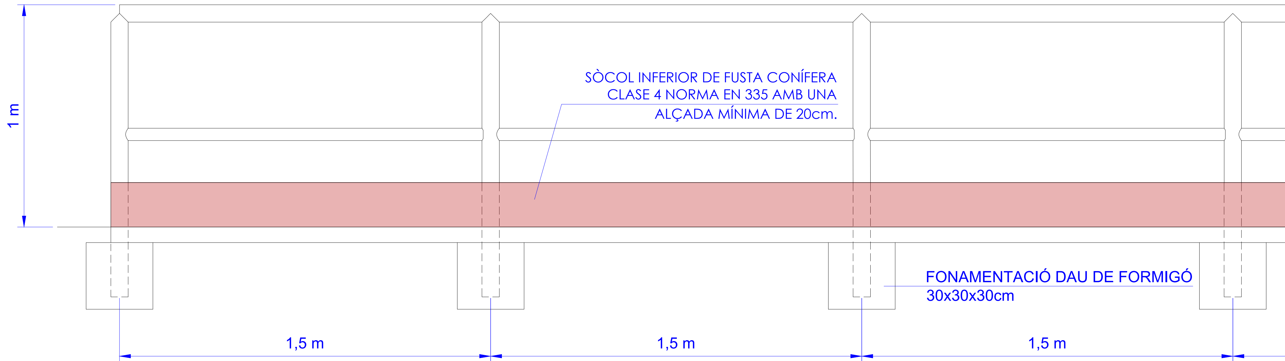
TANCA PERIMETRAL
