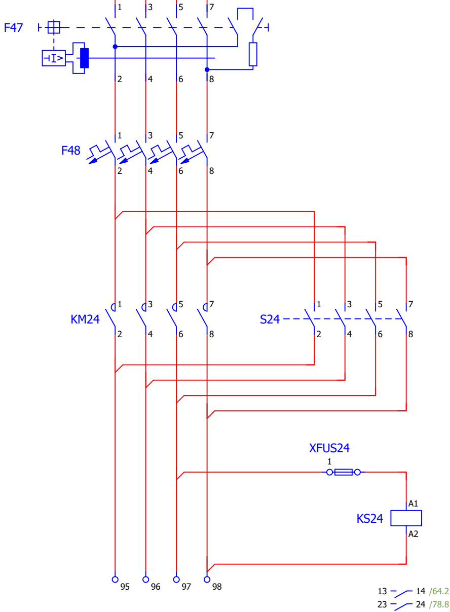
Circuit assolellat 16
