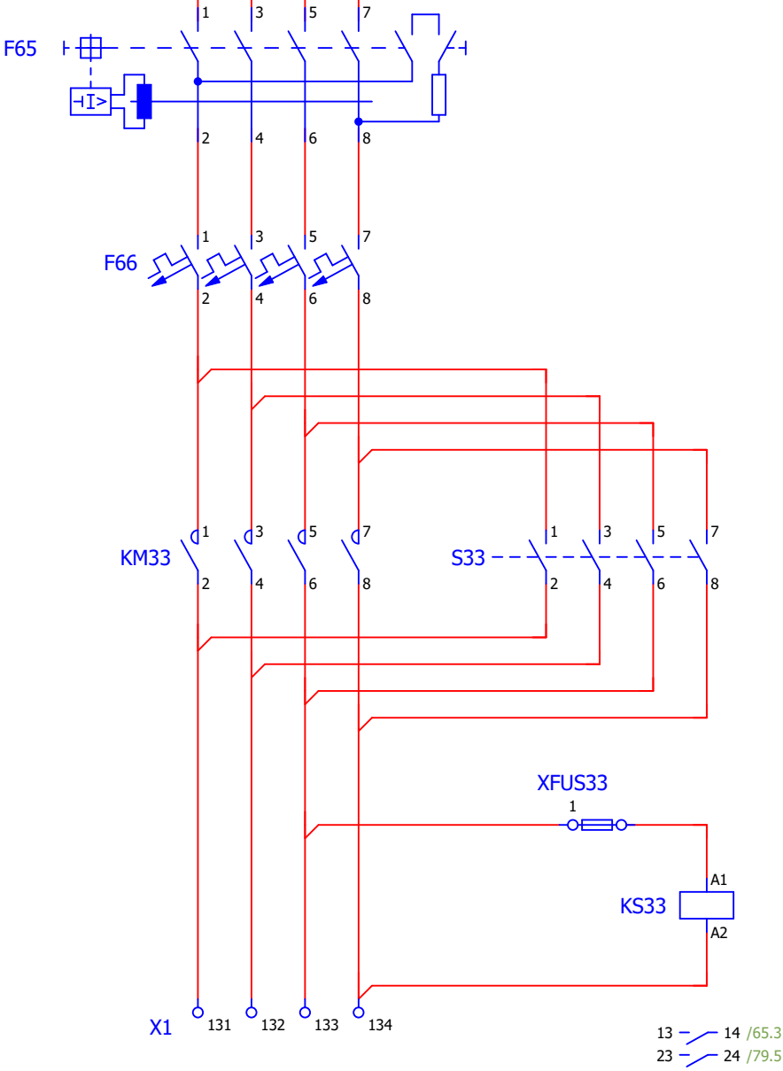
Circuit crepuscular 1
