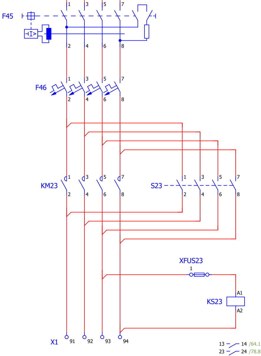
Circuit assolellat 15
