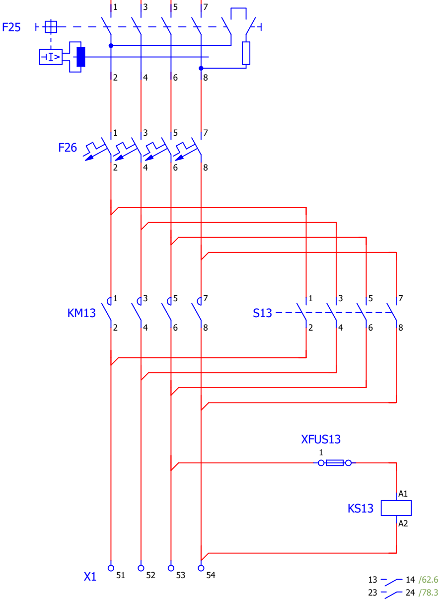
Circuit assolellat 5
