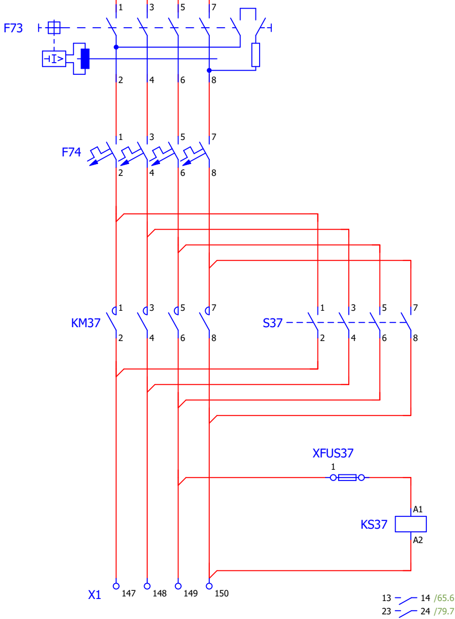
Circuit crepuscular 5
