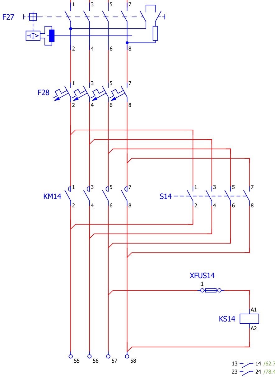
Circuit assolellat 6
