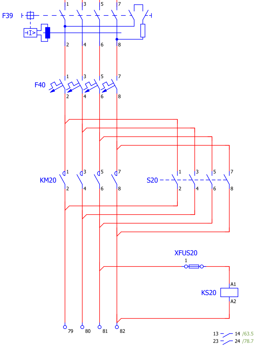
Circuit assolellat 12
