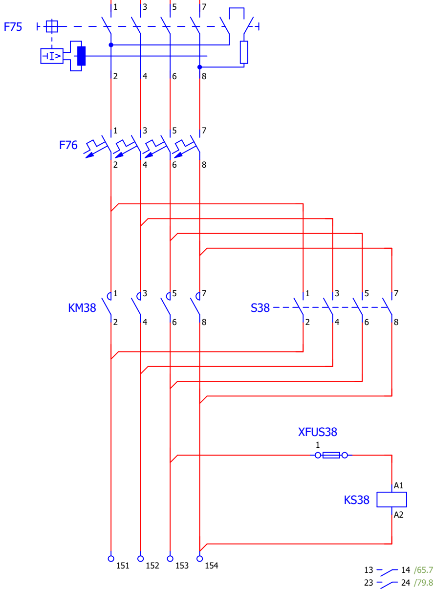
Circuit crepuscular 6
