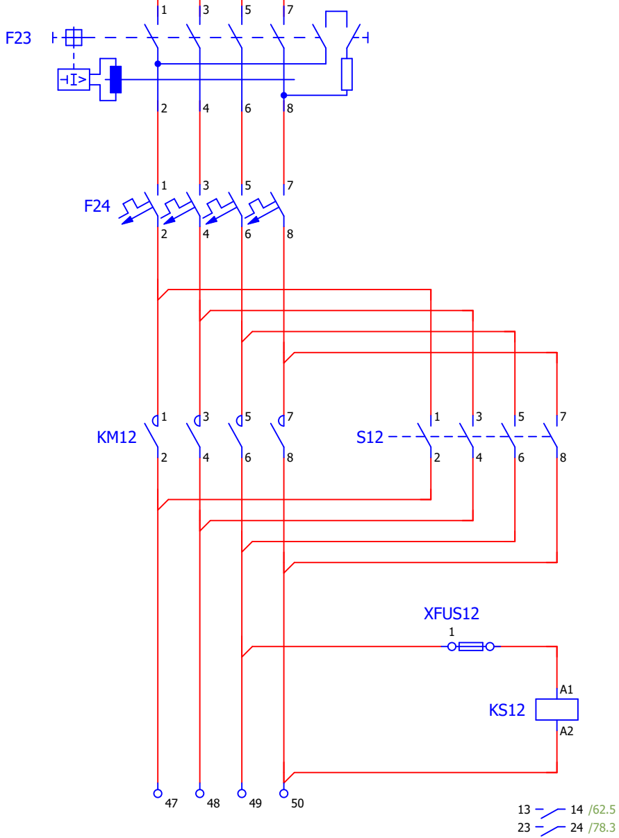
Circuit assolellat 4
