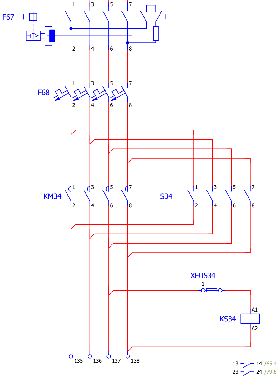
Circuit crepuscular 2
