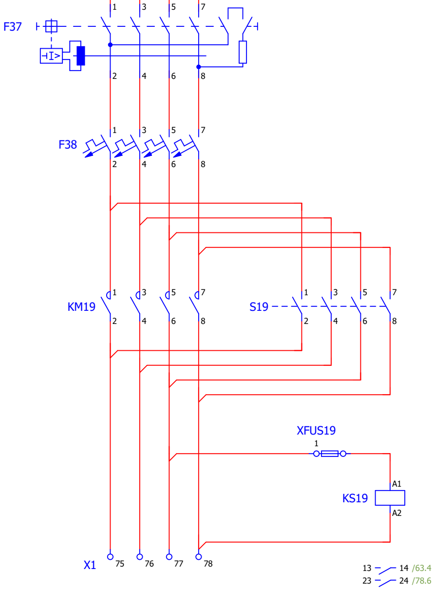
Circuit assolellat 11
