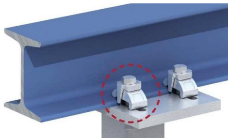
Grapes Lindapter
