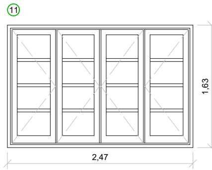
Finestra abatible
