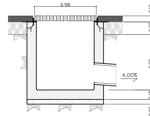
EMBORNAL RECOLLIDA AIGUES e: 1/25
