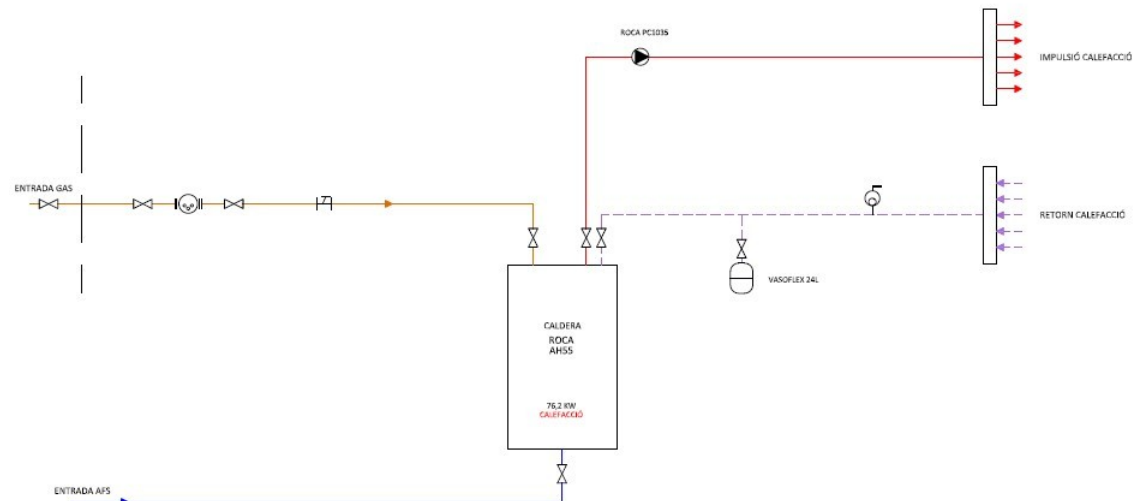
CALDERA GAS
