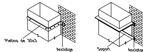
Soports de conductes rectangulars verticals a pared.
