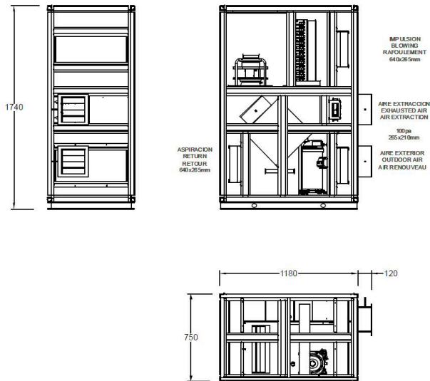
AIRPOOL 9 1800m 3 /h FREECOOLING 540m 3 /h
