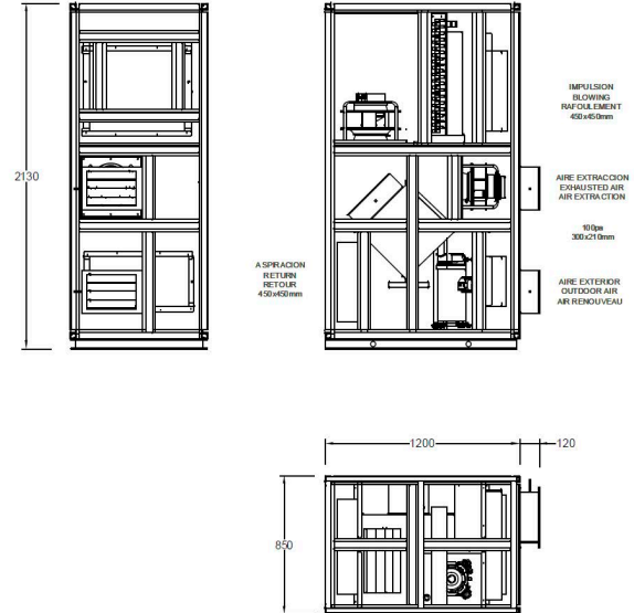
AIRPOOL 14 2500m 3 /h FREECOOLING 750m 3 /h
