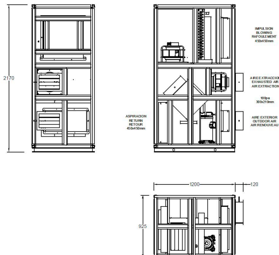
AIRPOOL 18 3800m 3 /h FREECOOLING 1140m 3 /h
