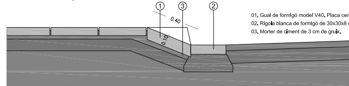
GUAL VEHICLES V40 - PLACA CENTRAL
