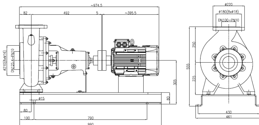
Bomba Likitech
