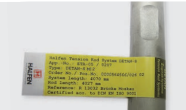
Label with product-specific data
