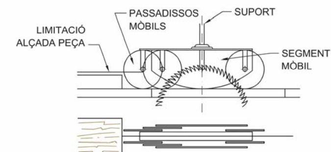
CARCASSES PROTECTORES
