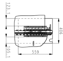
DETAIL A TYPE C12T SCALE 1:20 ECHELLE 1:20
