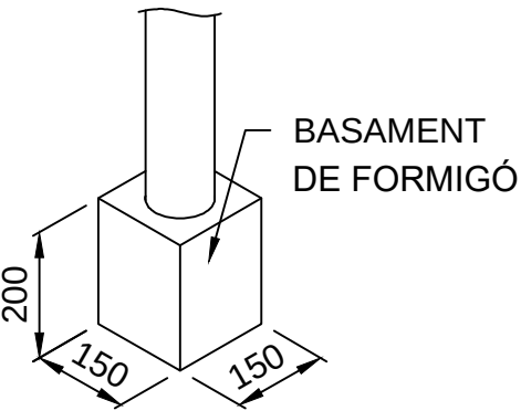
DETALL E 1/20 (A3) BASSAMENT PILONA
