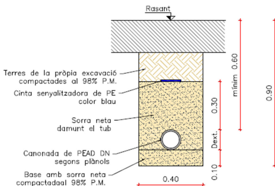
Figura 4. Detall Rasa canonada PEAD
