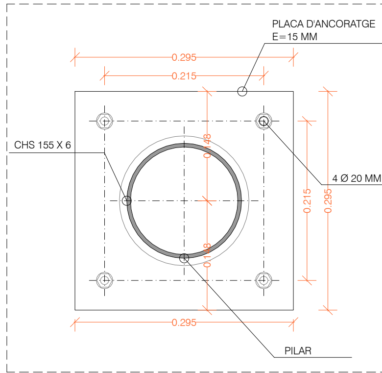
PLATINA INDIVIDUAL
