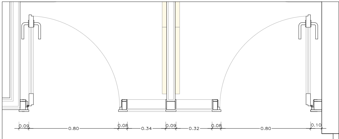
M3_MAMPARA
