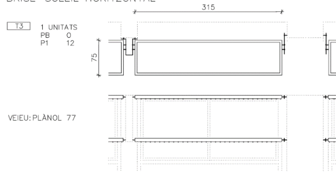
BRISE-SOLEIL HORIZONTAL
