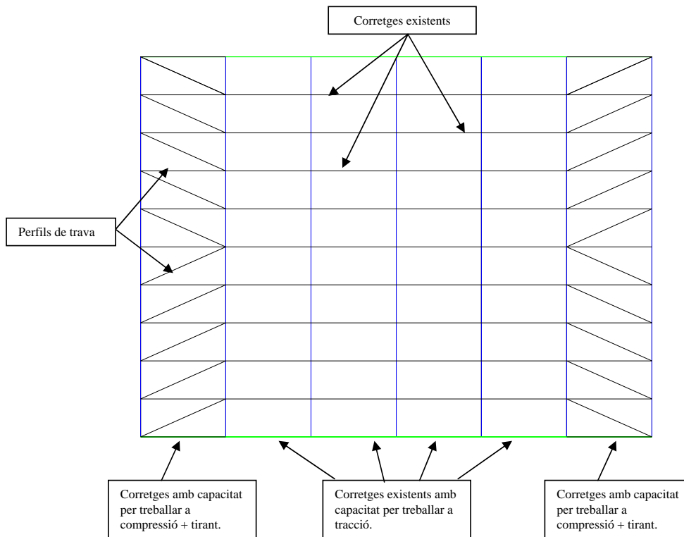
figura 9 – Planta detall noves triangulacions.
