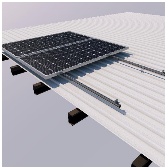
Figura 8 Estructura coplanar. Font: Sunfer Solar Mounting Systems
