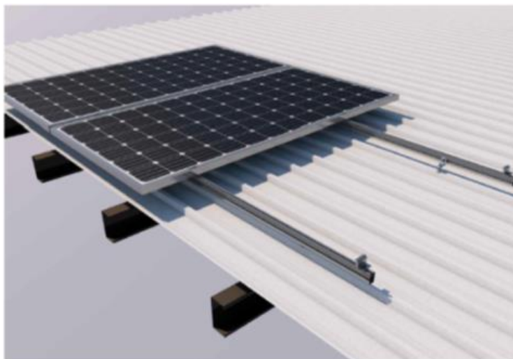
Figura 7 Estructura coplanar. Font: Sunfer Solar Mounting Systems
