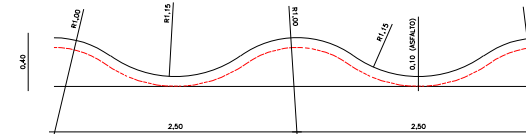
Detall Rollers
