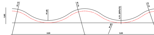
Detall Rollers
