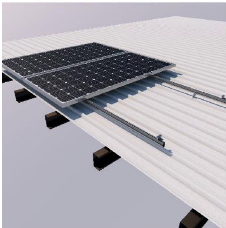
Figura 7. Estructura coplanar. Font: Sunfer Solar Mounting Systems
