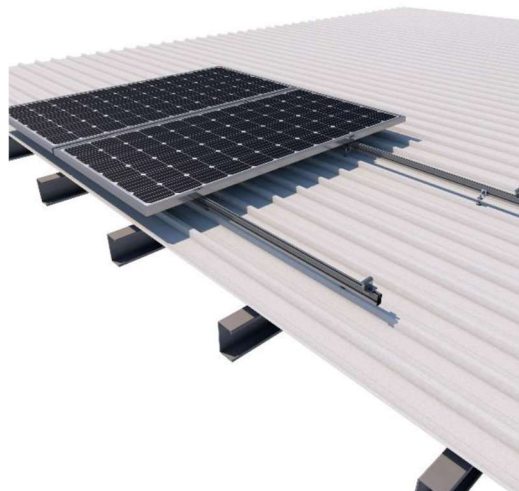
Figura 5 Estructura coplanar. Font: Sunfer Solar Mounting Systems
