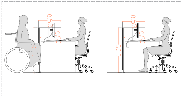
DETALLS
