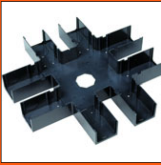
Fig. A: Removable grommetinserts can be slid into the outside of the compartments. The bottom of the Intercell junction box is provided with a hole that fits over an individual pedestal support of the Intercell structure.
