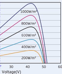
P-V CURVES OF PV MODULE(495W)
