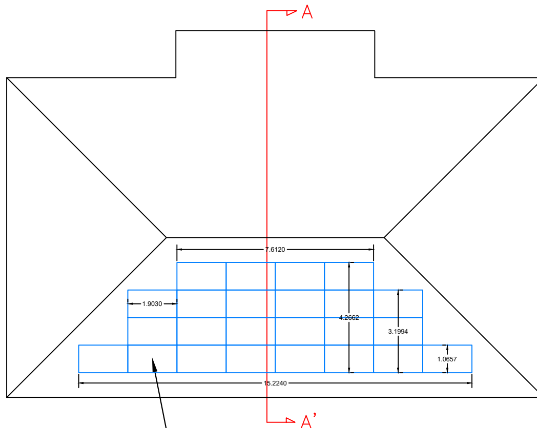
Mòdul fotovoltaic JINKO SOLAR JKM475-60HL4-V (1903x1134x30mm)
