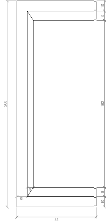
ALADO / FRONT VIEW
