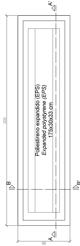
VISTA INFERIOR / BOTTOM VIEW
