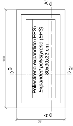
VISTA INFERIOR / BOTTOM VIEW
