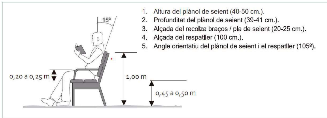
Figura 62. Dimensions del seient.
