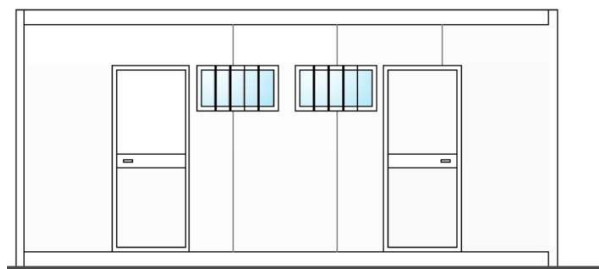
Façana principal
